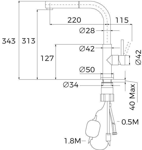
Swivel_Spout Easy_Quick
