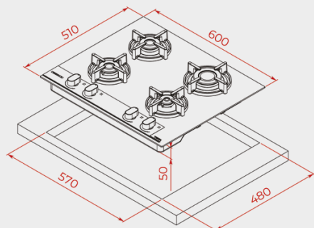
GBC 64 G 1 INFINITY
