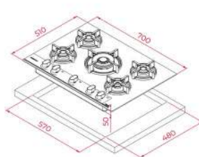
GBC 75 INFINITY G1
