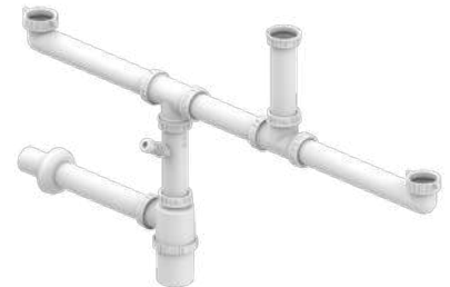
FITTINGS FOR 2 1/2 B: CONNECTION, SIPHON, PIPE TO WALL + DECORATIVE END CAP
