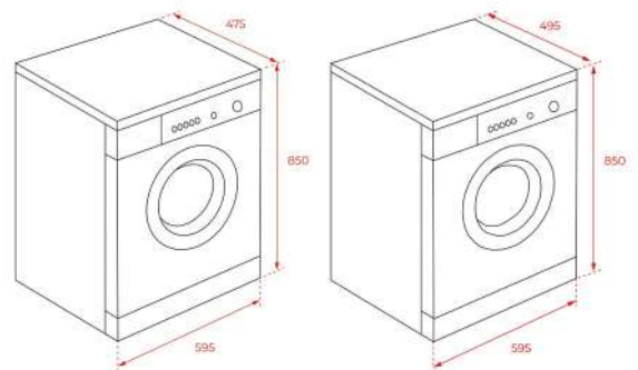
TK5 1480 WD SLIM WH
