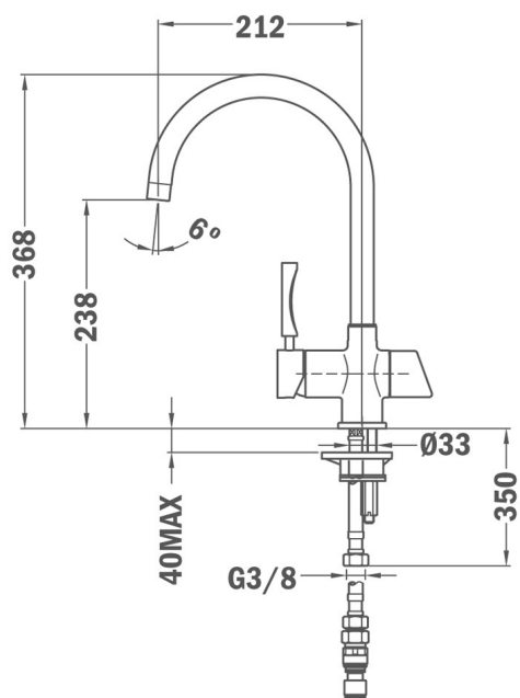
Swivel spout
