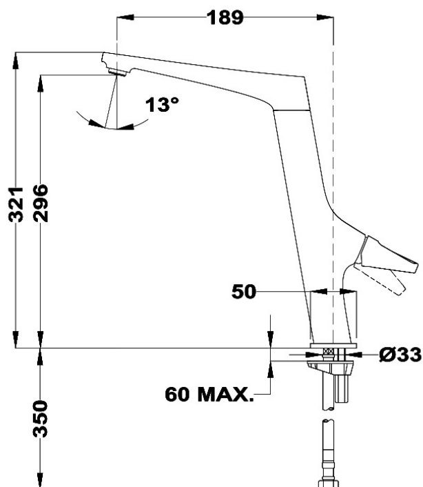
Swivel spout
