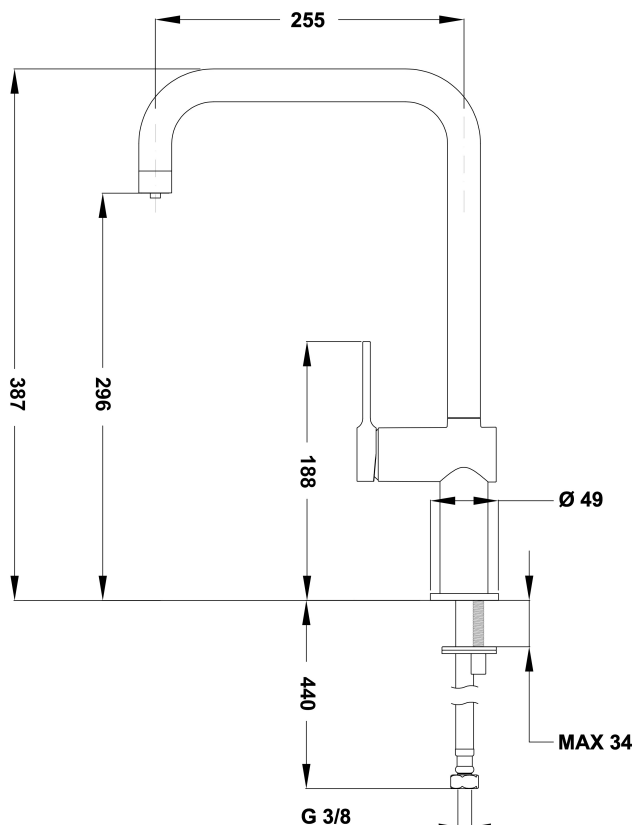
Swivel spout
