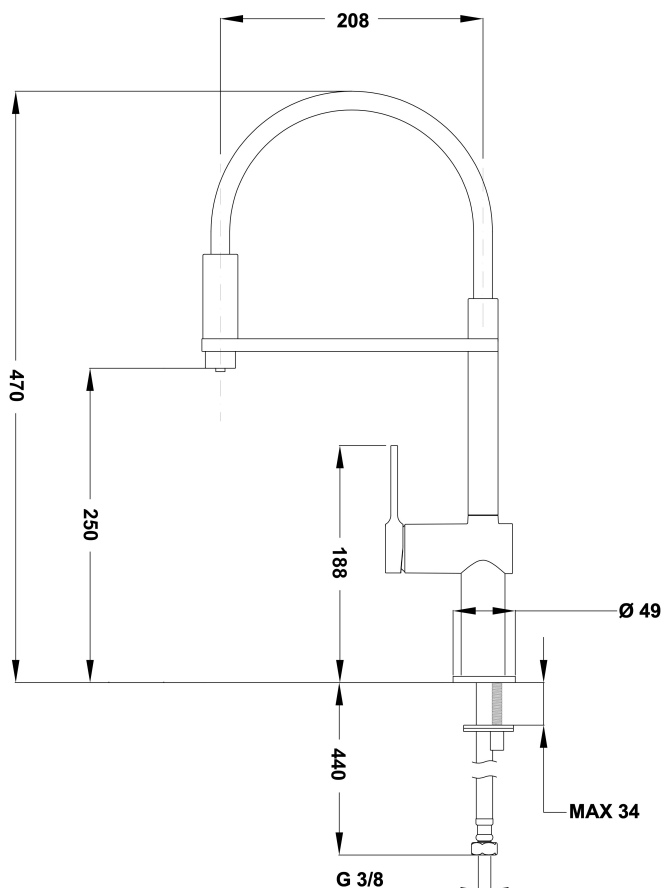
Swivel spout
