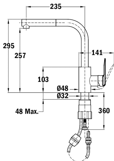
Swivel spout
