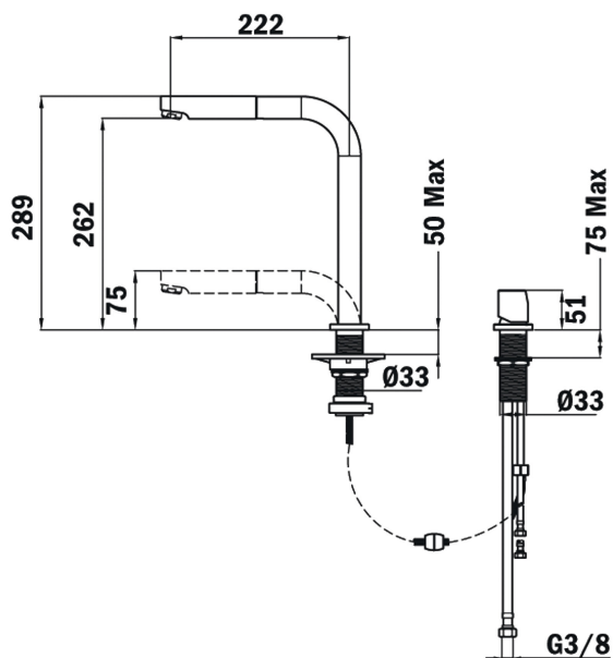
Swivel spout
