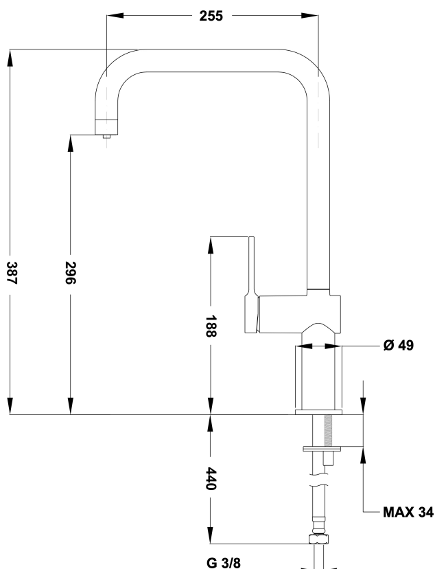
Swivel spout
