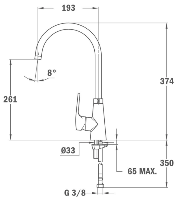
Swivel spout
