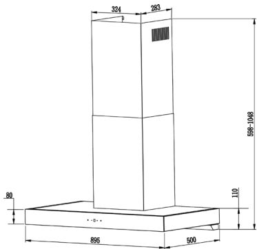
EXTERNAL DIMENSIONS Width 895mm
