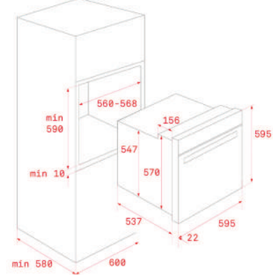
EXTERNAL DIMENSIONS Height 595mm Width 595mm Depth 559mm
