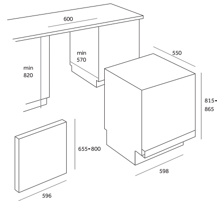
EXTERNAL DIMENSIONS Height 815/865mm Width 598mm Depth 550mm
