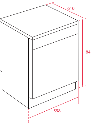
EXTERNAL DIMENSIONS Height 845mm Width 598mm Depth 610mm
