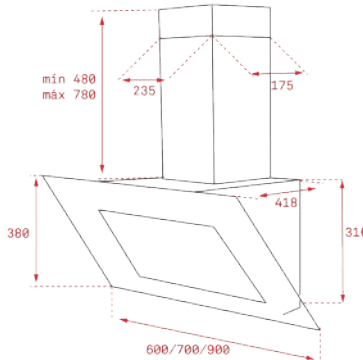
EXTERNAL DIMENSIONS Width 600mm/700mm/900mm
