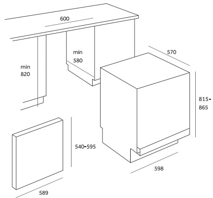
EXTERNAL DIMENSIONS Height 815/865mm Width 598mm Depth 570mm
