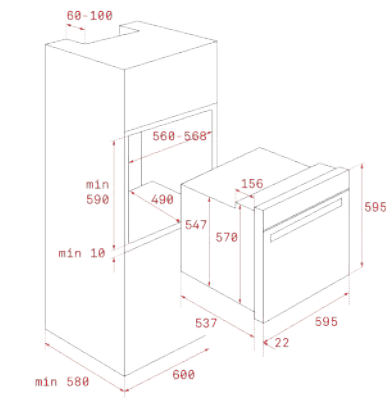
EXTERNAL DIMENSIONS Height 595mm Width 595mm Depth 559mm
