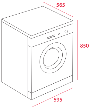
EXTERNAL DIMENSIONS Height 850mm Width 595mm Depth 565mm
