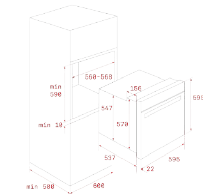
EXTERNAL DIMENSIONS Height 595mm Width 595mm Depth 559mm
