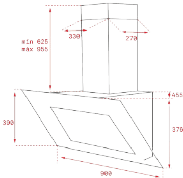
EXTERNAL DIMENSIONS Width 900mm
