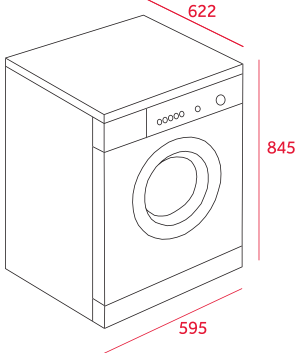
EXTERNAL DIMENSIONS Height 845mm Width 595mm Depth 622mm
