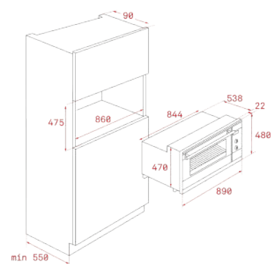
EXTERNAL DIMENSIONS Height 480mm Width 890mm Depth 560mm
