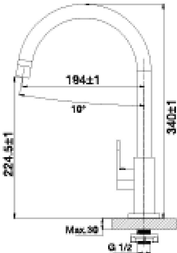
Swivel spout
