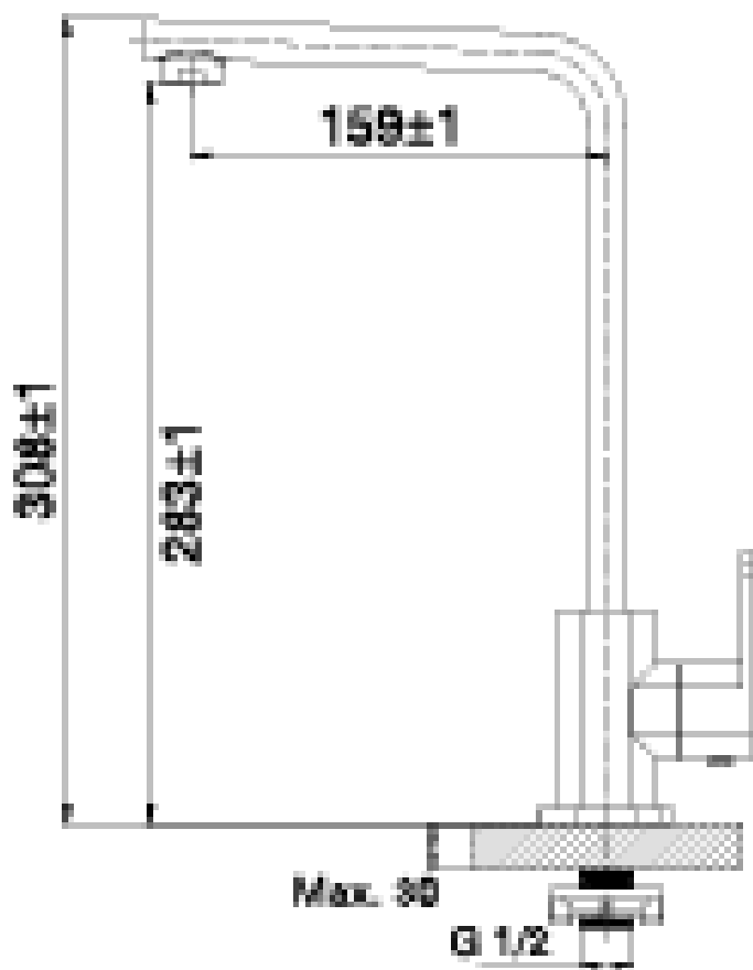
Swivel spout
