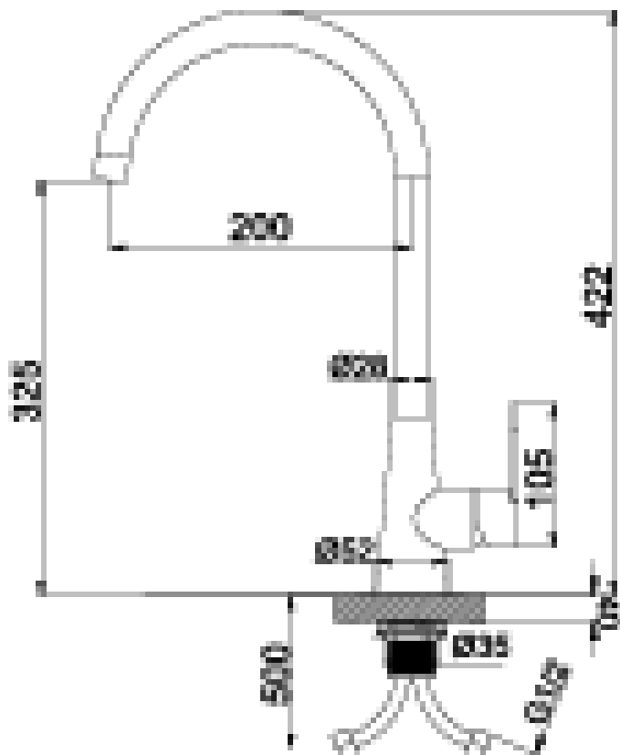
Swivel spout
