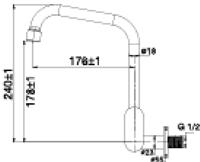
Swivel spout
