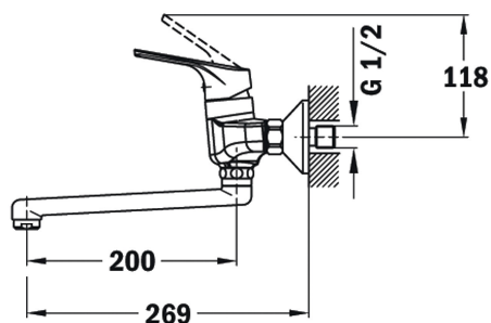
Swivel spout
