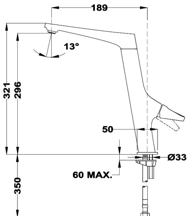
Swivel spout
