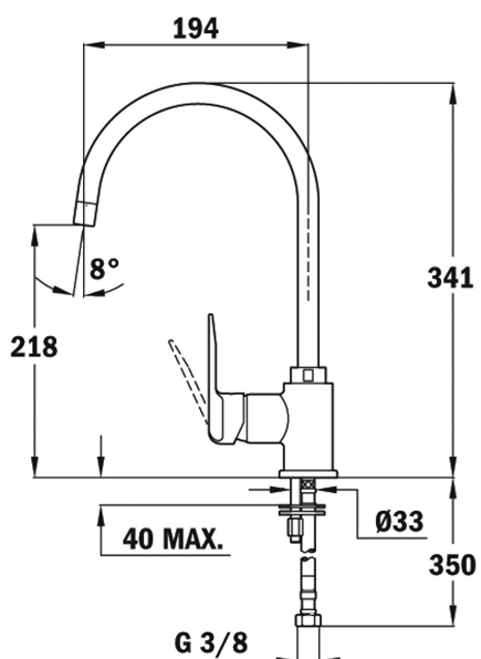
Swivel spout
