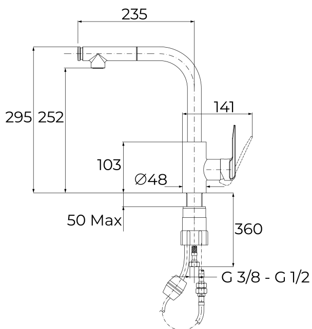
Anti-Scale Aerator
