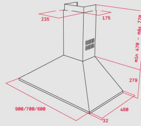
DBB 90/70/60 INOXIDABLE
