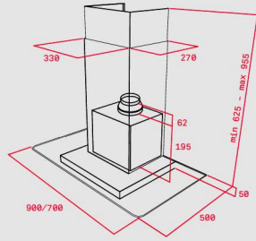
DG 980/780 CRISTAL
