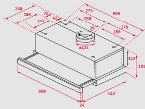
TL 6310 INOX.
