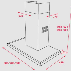
DJE 90/70/60 INOXIDABLE
