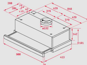
TL 9310 INOX.
