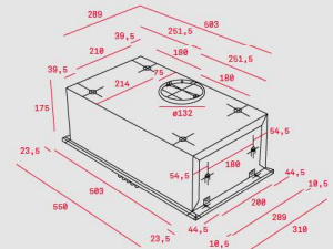
GFH 55 INOXIDABLE
