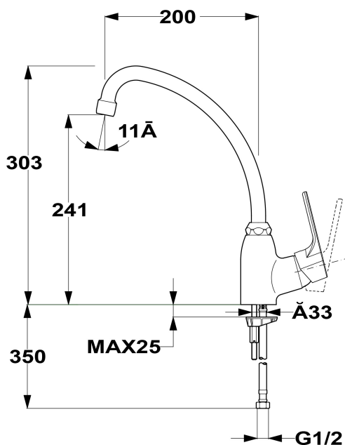
Swivel Spout
