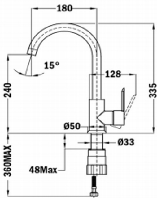
Swivel Spout
