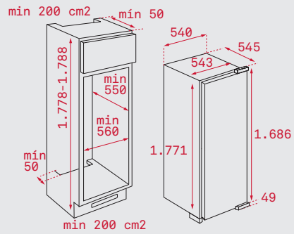
ARTIC TGI2 200 NF
