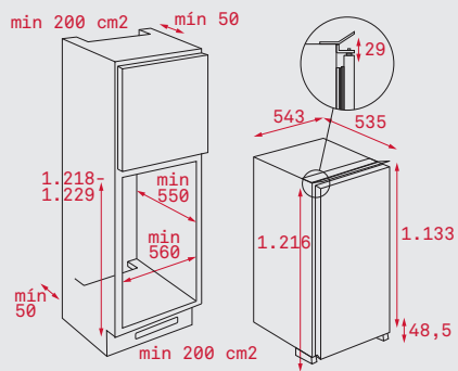
ARTIC TKI4 235 · ARTIC TKI4 215
