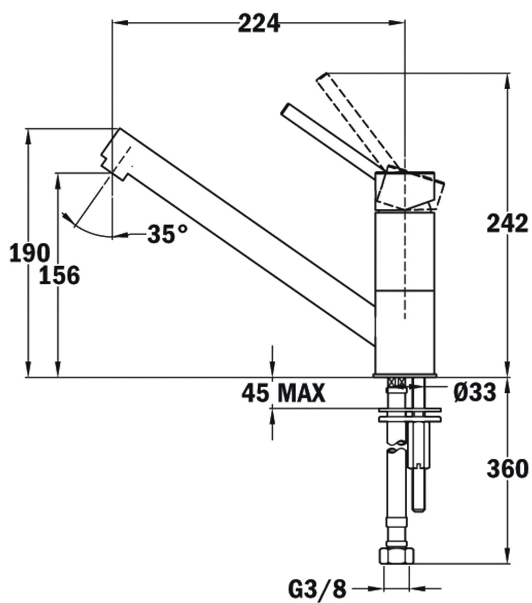
Swivel spout
