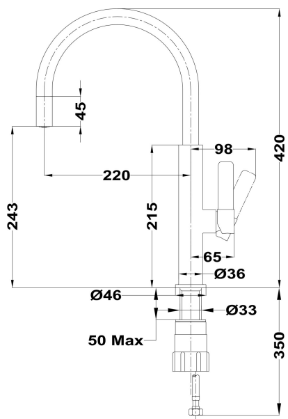
Swivel Spout
