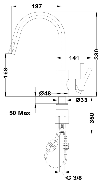
Swivel Spout
