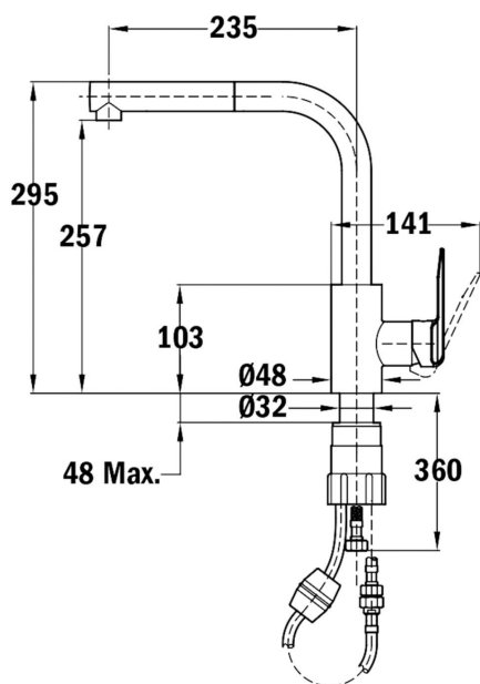
Swivel Spout
