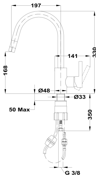
Swivel Spout
