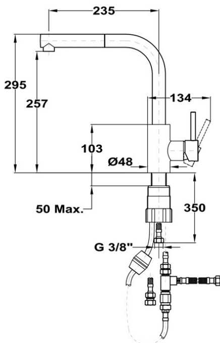
Swivel Spout
