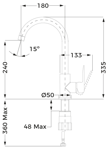
Swivel Spout
