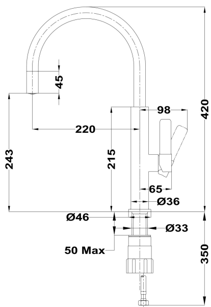
Swivel Spout
