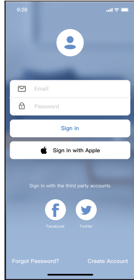
iOS
