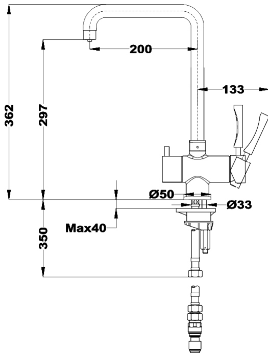
Anti-scale aerator
